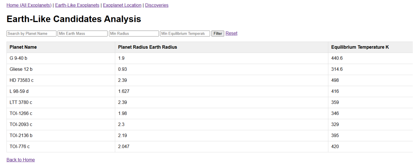
Figure 34. Earth Like exoplanets WHERE Planet_Radius_Earth_Radius BETWEEN 0.5 AND 2.5 AND Equilibrium_Temperature_K BETWEEN 150 AND 500
